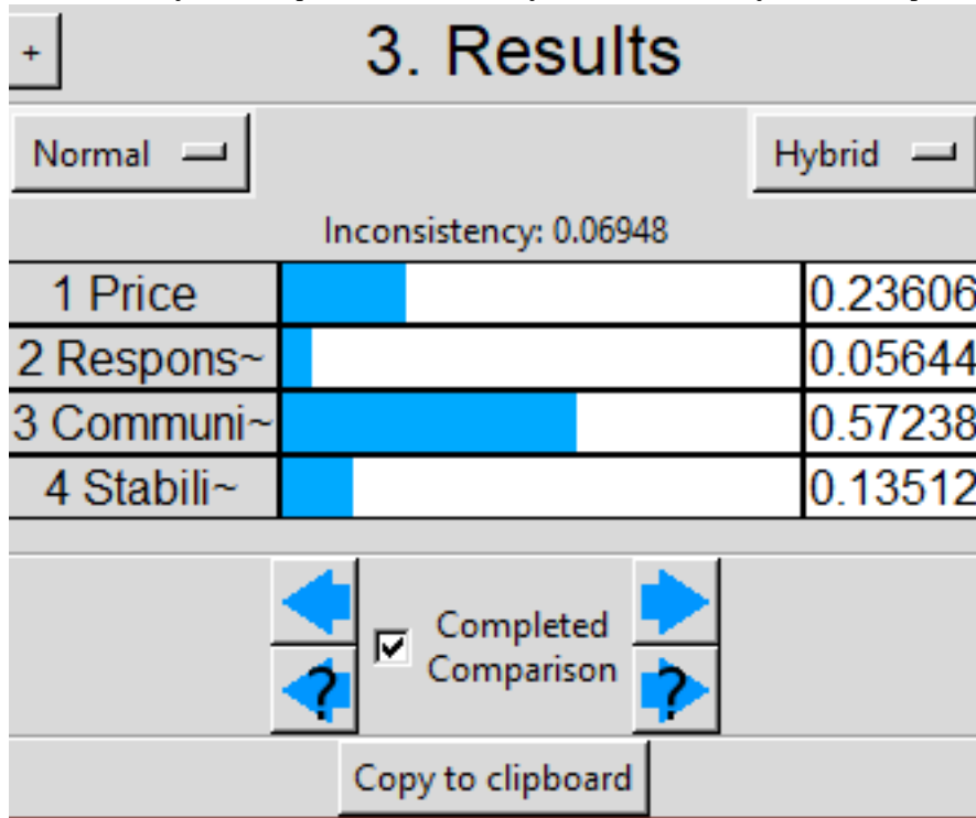
Figure 3: Inconsistency of Pairwise comparisons.
