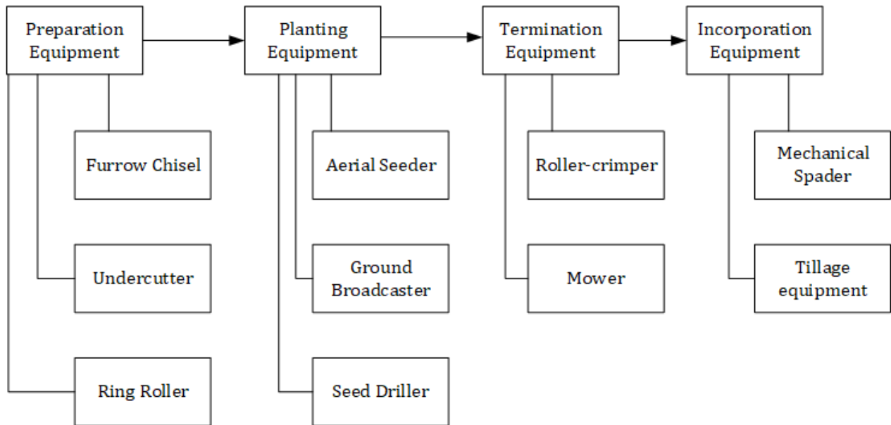
Figure 3: Mechanized Cover Crop Farming Equipment
