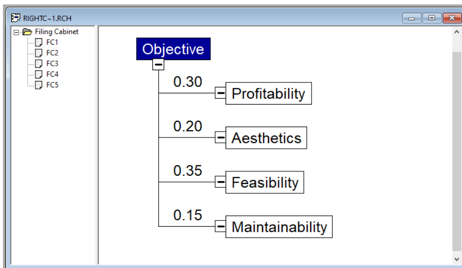
Figure 4: RightChoice Model.
