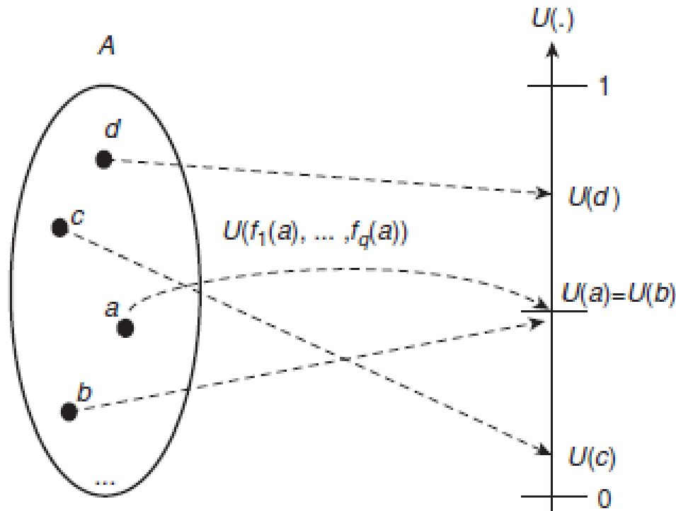
Figure 1: Representation of the ranking of the set A using the MAUT model [17].
