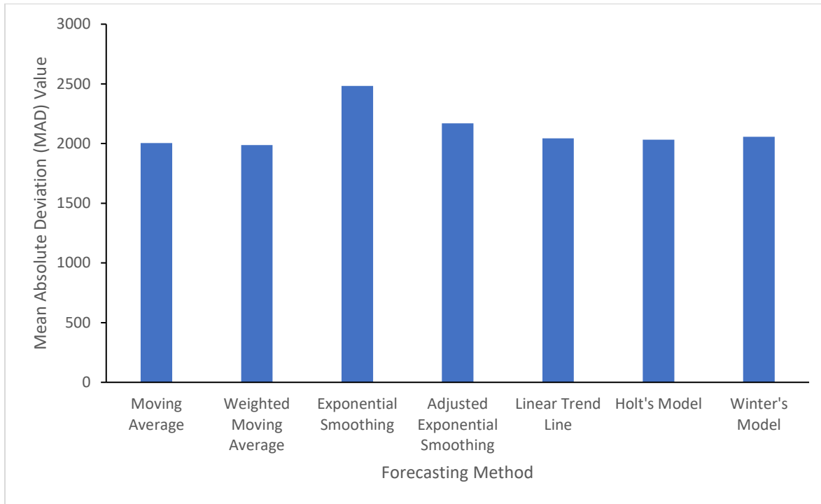
Figure 8: Comparison of Mean Absolute Deviation (MAD) values for various 50cl bottled water forecasting methods.
