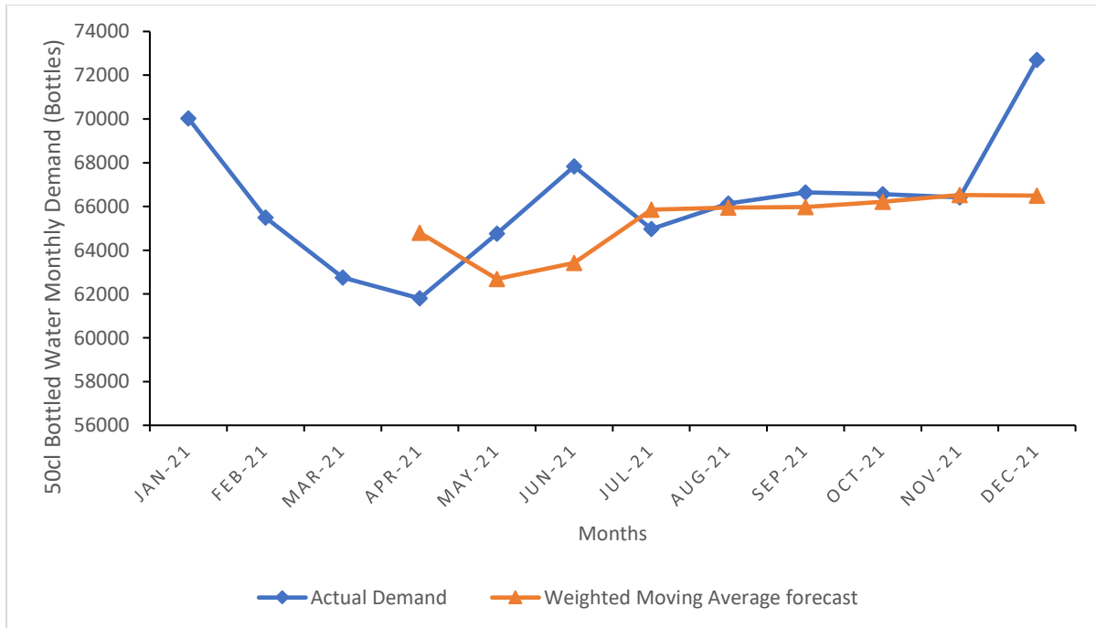
Figure 2: Plot of actual 50cl bottled water monthly demand and the 3-month Weighted Moving Average forecast against months of the year.
