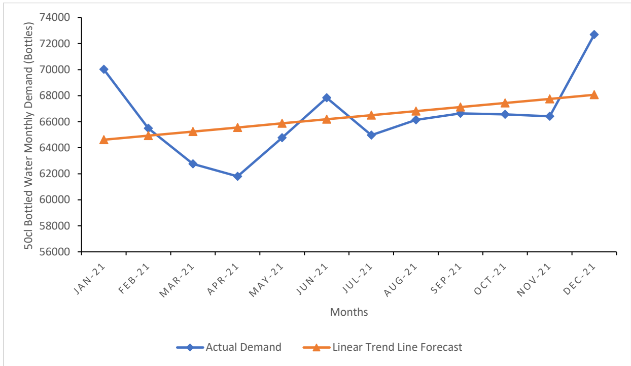
Figure 5: Plot of actual 50cl bottled water monthly demand and the Linear Trend Line forecast against months of the year.
