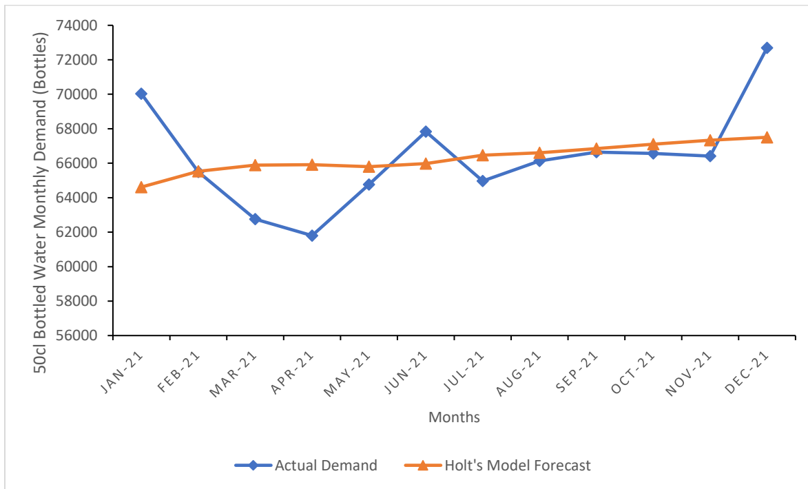
Figure 6: Plot of actual 50cl bottled water monthly demand and the Holt’s model forecast against months of the year.
