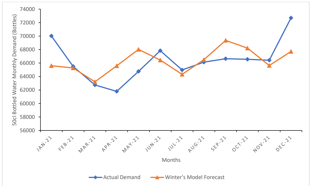
Figure 7: Plot of actual 50cl bottled water monthly demand and the Winter’s model forecast against months of the year.
