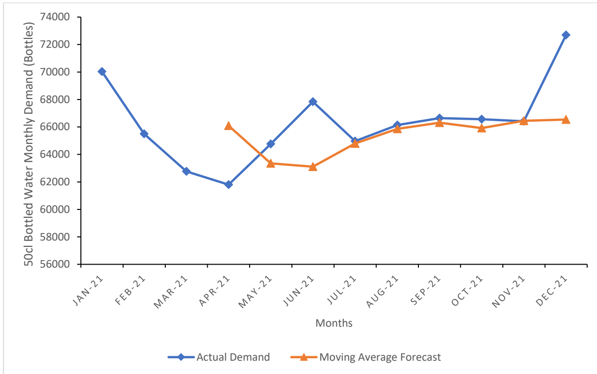
Figure 1: Plot of actual 50cl bottled water monthly demand and the 3-month Moving Average forecast against months of the year.
