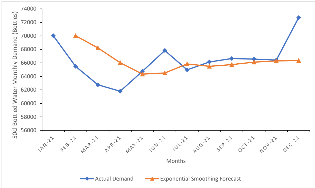
Figure 3: Plot of actual 50cl bottled water monthly demand and the Exponential Smoothing forecast against months of the year.
