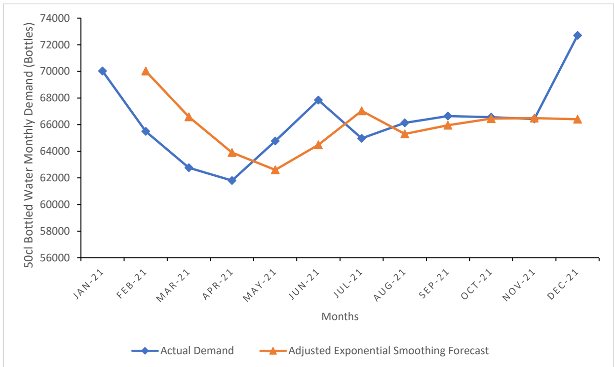
Figure 4: Plot of actual 50cl bottled water monthly demand and the Adjusted Exponential Smoothing forecast against months of the year.
