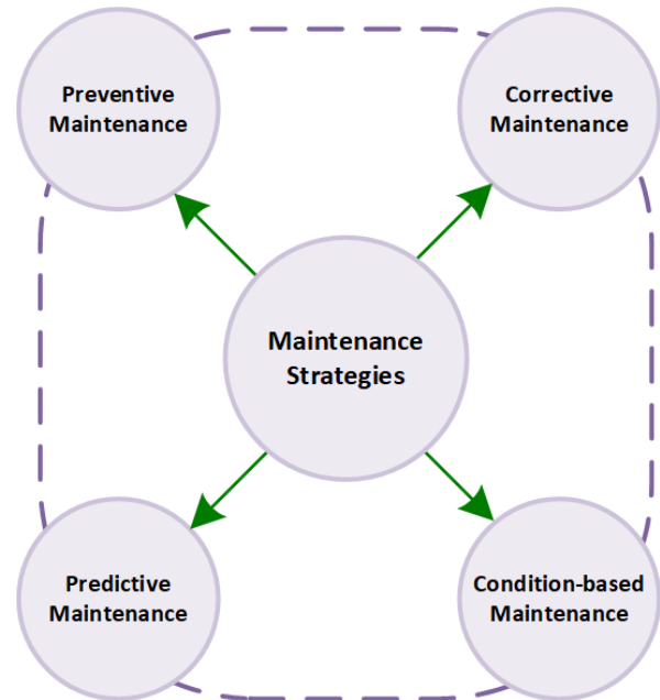
Figure 2: Maintenance strategies.
